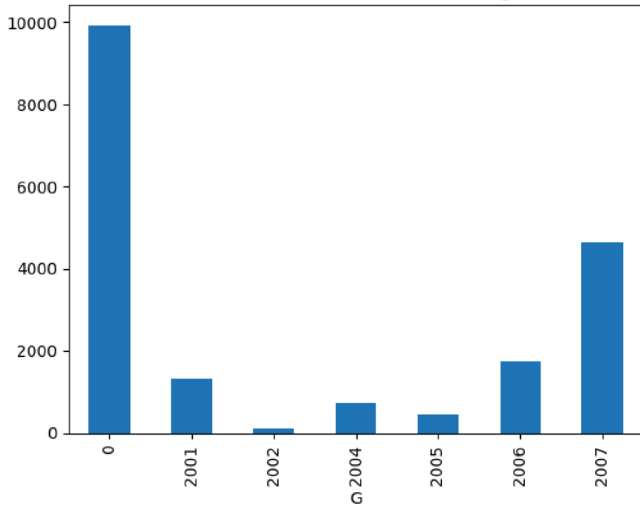
Distribution of Treatment Timing
